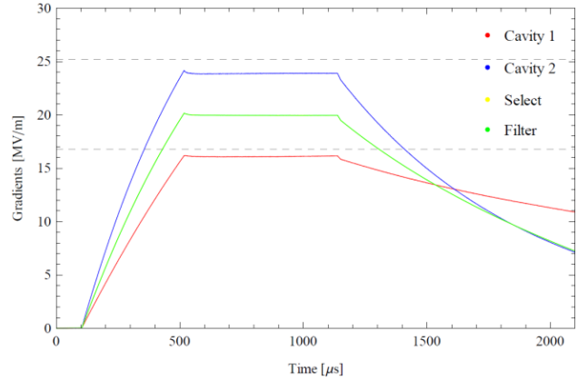
Figure 8: Gradients [MV/m] versus time [ \mu\text{s} ] during P_k Q_L operation. The dashed lines indicate the virtual quench limits.
