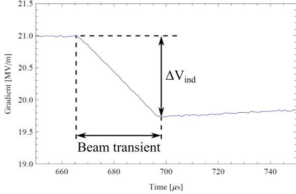
Figure 2: Cavity 1 gradient [MV/m] versus time [ \mu\text{s} ] during the flattop covering the beam transient, during which beam loading induces the gradient drop \Delta V_{\text{ind}} .
