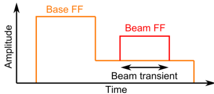
Figure 3: Schematic of the amplitude versus time for a base FF table (orange) and a beam FF table (red).
