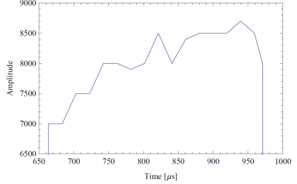
Figure 4: Amplitude versus time [ \mu\text{s} ] of automatically generated beam FF table.
