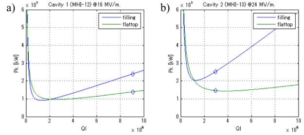
Figure 7: Power [kW] versus Q_L for a) cavity 1 and b) cavity 2. Working points are marked by blue diamonds.
