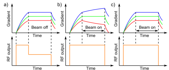
Figure 6: Schematic of cavity 1 (red), cavity 2 (blue), and vector sum (green) gradients with corresponding RF output for a) nominal operation without beam, b) nominal operation with beam, and c) P_k Q_L operation with beam.
