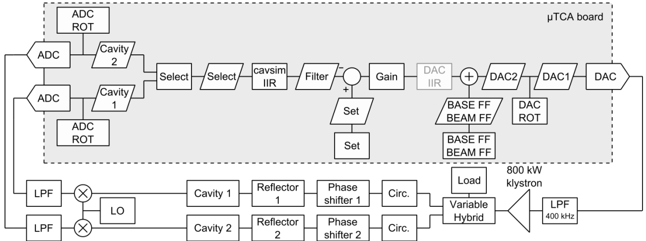
Figure 1: Schematic of the digital LLRF feedback loop controlling two superconducting cavities at STF. Hardware and software components are represented by squares, data channels accessible on the \mu TCA board via EPICS by rhombi.
