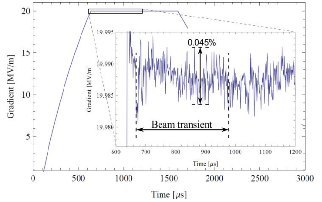
Figure 5: Vector sum gradient [MV/m] versus time [ \mu\text{s} ] after automated generation of beam FF table.
